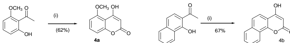
Scheme 3: Reaction scheme for the synthesis of derivatives of 4-hydroxycoumarin ( 4a and 4b ).
